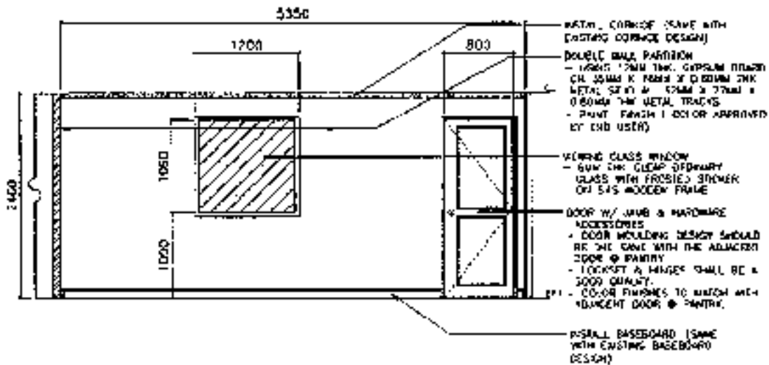
ELEVATION @ SECTION B SCALE 1" = 3' 0"
