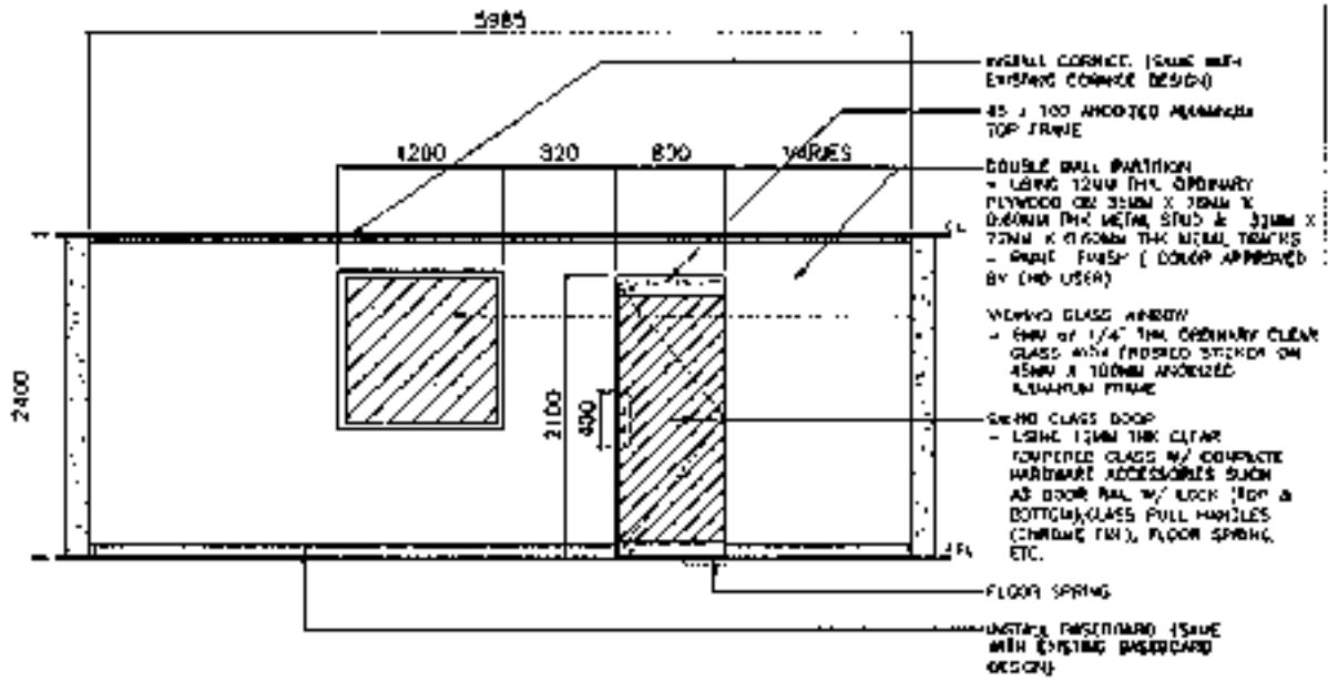
ELEVATION @ SECTION A SCALE 1" = 3' 0"
