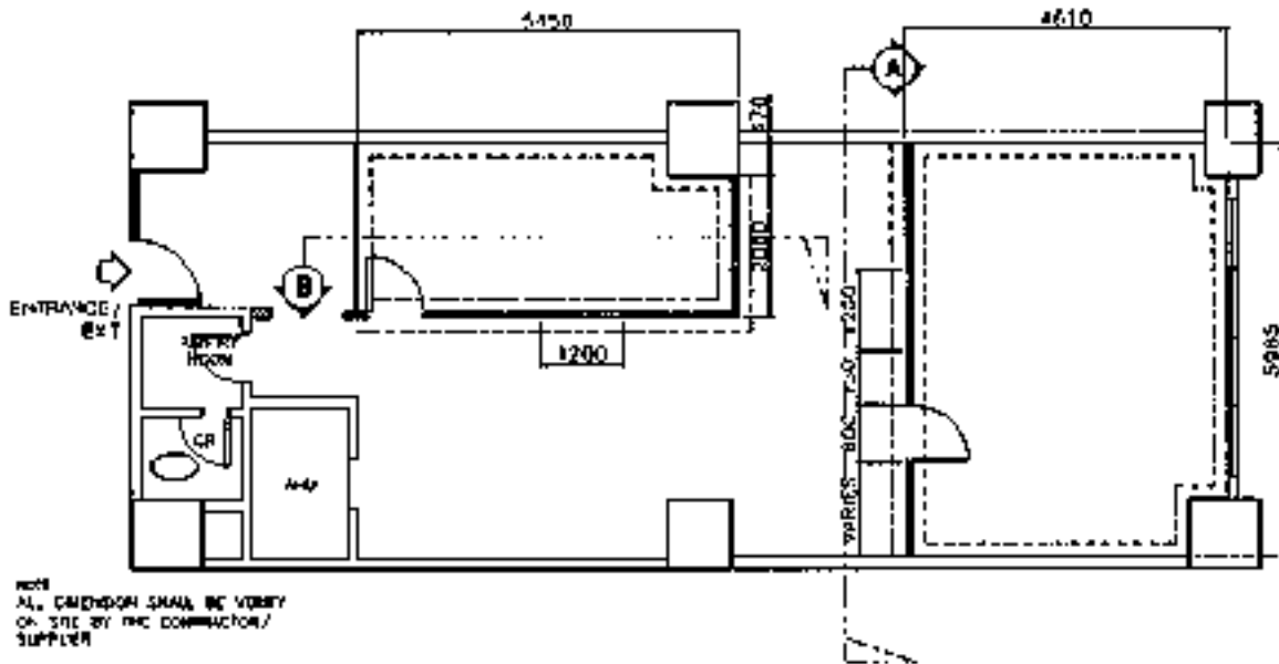
PROPOSED PLAN SCALE: 1/4" = 1'-0"
