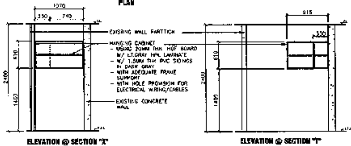
PROPOSED HANGING CABINET @ PANTRY ROOM
